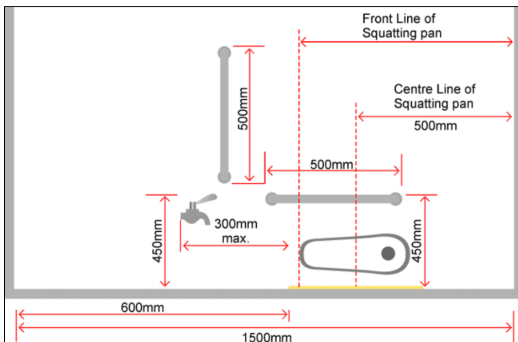
Figure 16-8. Side view of accessible squatting toilet
