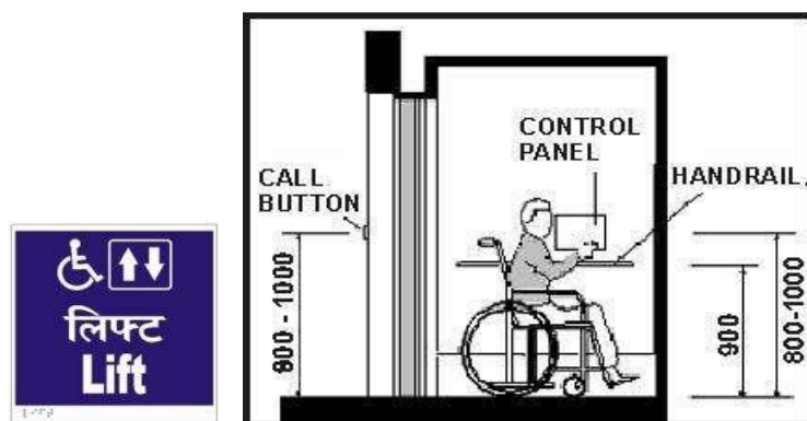
Figure 10-1. Lift Signage, Internal Dimensions and Control Panel
