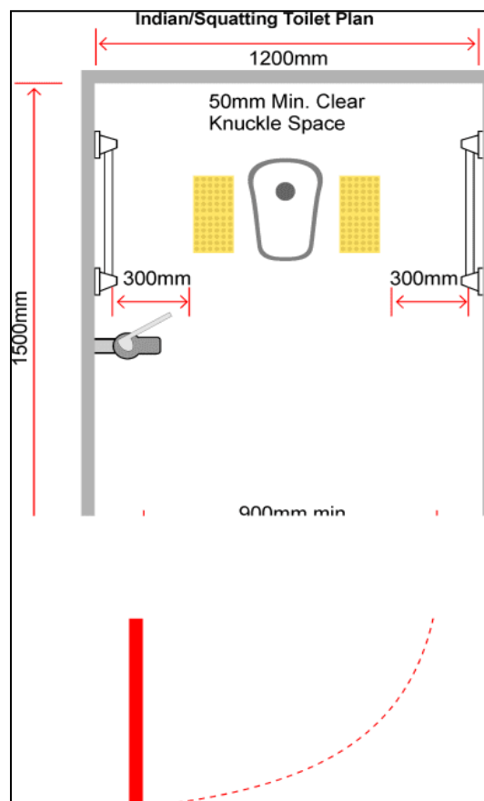
Figure 16-7. Layout and dimensions of accessible squatting seat
